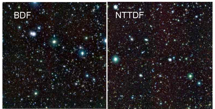
Fig. 1. Colour-composite image of the BDF (left) and NTTDF (right) fields, created using the weighted mean of Hawk-I Y , J and K images as red, the FORS2 Z as green, and the weighted mean of FORS1/FORS2 optical images as blue.
