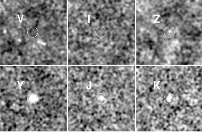
Fig. 4. Thumbnails showing the stacked images of the 15 high-redshift candidates selected in the GOODS1, GOODS2, BDF and NTTDF fields. The observed bands are shown in the legends.
