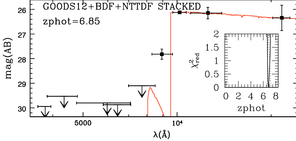
Fig. 5. Best-fit SED to the stacked photometry, with relevant photometric redshift at z = 6.85 .
