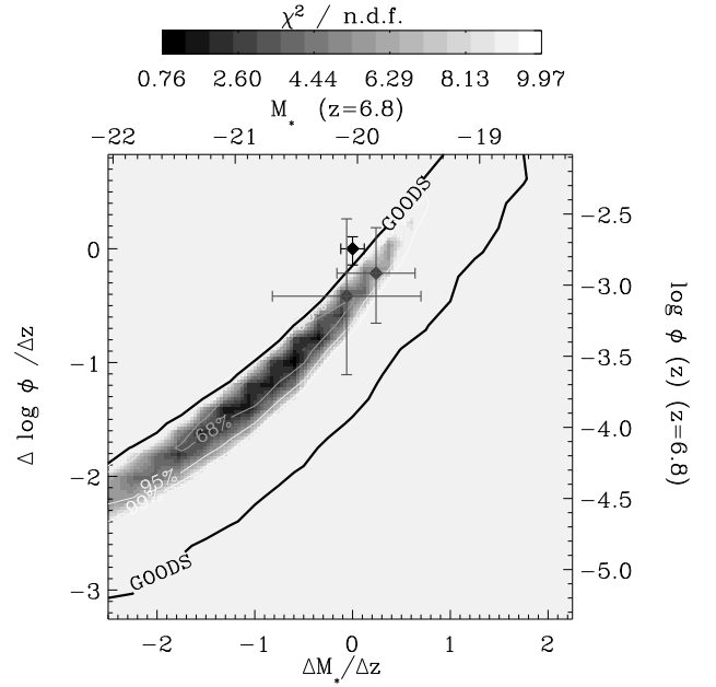
Fig. 8. \chi^2 contour levels for the d\log(\phi)/dz , M'_* parameters derived for the Schechter-like LF considering all the four Hawk-I fields. The lower and left axis refer to the evolutionary terms M'_* and d\log(\phi)/dz with respect to the best-fit z=6 parameters of McLure et al. (2009) (black point and errorbars). The upper and right axis refer to the M_* and \phi values at the median redshift estimated for our sample ( z=6.8 ). Grey points and errorbars mark the position of the z \sim 7 best fit parameters by Ouchi et al. (2009a) and by Bouwens et al. (2008). The black solid line indicates the 99% c.l. region estimated on the basis of the two GOODS-South pointings only (C10).
