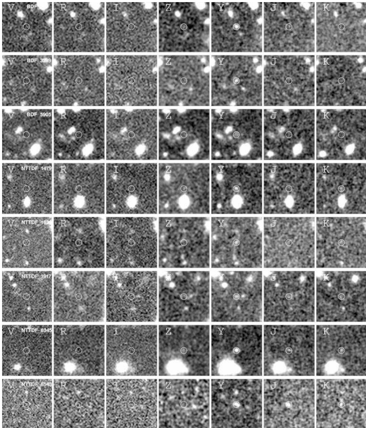
Fig. 3. Thumbnails showing the images of the 8 selected high-redshift candidates in the different observed bands.
