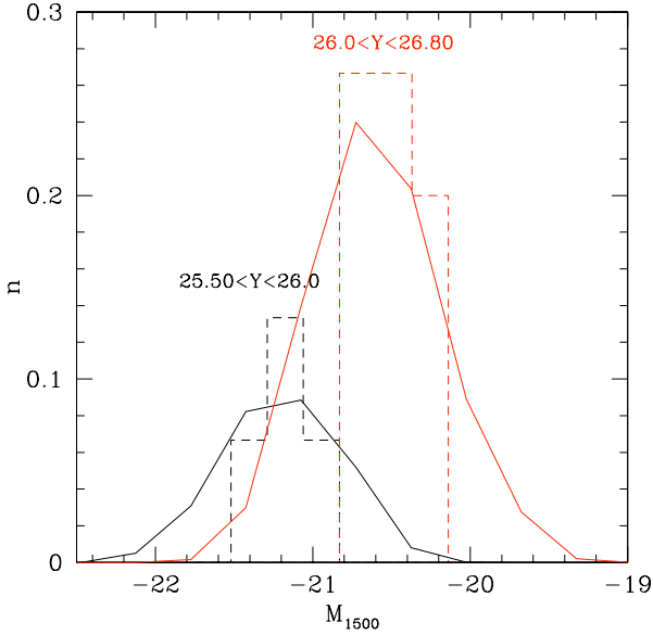
Fig. 7. The normalized distribution of UV continuum magnitudes (estimated from the average Y - M_{1500} relation) for the 15 Hawk-I candidates divided in two bins (dashed histograms). The solid curves show the expected distributions of UV magnitudes for objects in the same observed ranges when photometric uncertainties are taken into account through MonteCarlo simulations.
