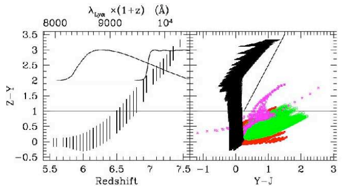
Fig. 2. Left: Z - Y colour of star forming galaxies as a function of redshift. In the upper part, the efficiency curve of the two filters is shown, computed at observed wavelength of a Lyman- \alpha emission at the corresponding redshift. Right: Z - Y vs. Y - J colour diagram showing the expected colours of LBGs (same as in left panel, black points), passively evolving galaxies (red squares) and reddened starbursts (green circles) at 1.5 < z < 4 and cool dwarf stars from the templates of Tsuji et al. (2004) (magenta stars). Galaxy colours are computed according to CB07 models, see text for details on the adopted parameters. In both panels lines indicate the relevant colour selection criteria discussed in Sect. 3
