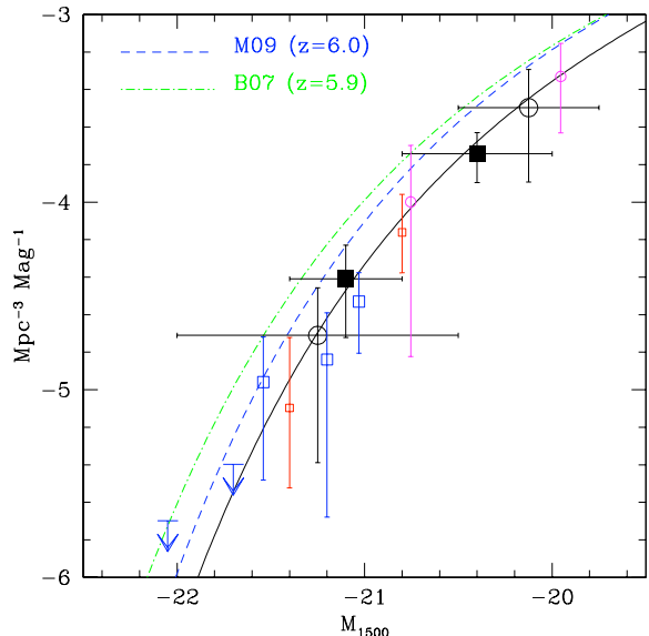
Fig. 6. Number densities in two rest-frame magnitude intervals estimated for our Hawk-I data set in a stepwise form with a standard Y -UV conversion of the observed number counts as discussed in the text (black filled squares), or with a \chi^2 method considering also photometric and model uncertainties (black empty circles). Other points are from Bouwens et al. (2010a) (NICMOS, red empty squares), Ouchi et al. (2009a) (SUBARU, blue empty squares and upper limits) and Oesch et al. (2010) (WFC3-UDF, magenta empty circles). For a comparison we show the recent determinations of the LF at z \sim 6 by Bouwens et al. (2007) (B07, green dot-dashed line) and McLure et al. (2009) (M09, blue dashed line). The black solid line is the best-fit LF obtained by combining the stepwise points shown in the figure with new determinations of the binned densities from WFC3-UDF and WFC3-ERS data (Grazian et al. in preparation).
