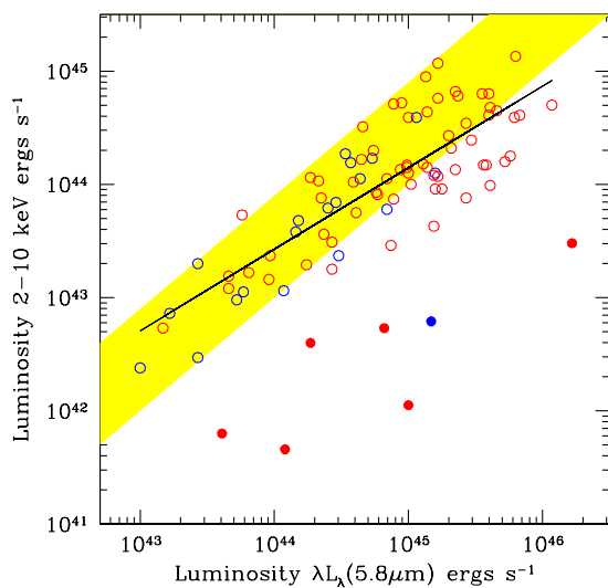
FIG. 5.— The 2-10 keV luminosity (not corrected for obscuration) as a function of the 5.8\mu\text{m} luminosity for 2 samples of type 1 AGN: C-COSMOS (red symbols) and CDF-S (blue symbols). For most of the points this 2-10 keV luminosity can be considered representative of the intrinsic X-ray luminosity. Filled circles identify seven outliers with small X-ray luminosity with respect to their infrared luminosity, suggesting X-ray absorption in these sources, and therefore that the intrinsic X-ray luminosity is likely underestimated in these cases. For this reason these sources have been excluded from the analysis. The black solid line is the best fit linear regression in eq.1. The shaded region is the linear extrapolation of the intrinsic X-ray-to-mid-infrared luminosity ratio found in the local Universe (Lutz et al. 2004).
