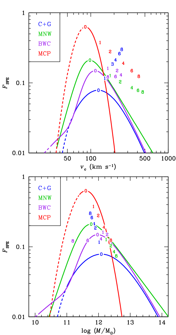
Figure 2. Star formation efficiency, F_{\text{SFE}} , of our analytical galaxy formation models versus halo circular velocity ( top ) and mass ( bottom ) at z=0 . The blue , green and purple curves respectively show F_{\text{SFE}} = m/(f_b M) for models C+G (Cattaneo et al. 2011 with Gnedin 2000, eqs. [5], [6] and [7]), MNW (Moster et al. 2013, eqs. [8] and [9]), and BWC (Behroozi et al. 2013, eqs. [10], [11], [12], and [13]). For model MCP (Mutch et al. 2013, eqs. [15] and [16], red curve ), F_{\text{SFE}} = 0.7 \dot{m}/(f_b \dot{M}) . The dashed portions of the curves indicate where the models are extrapolations. The numbers indicate the position of the peak star formation efficiency at the corresponding redshift.
