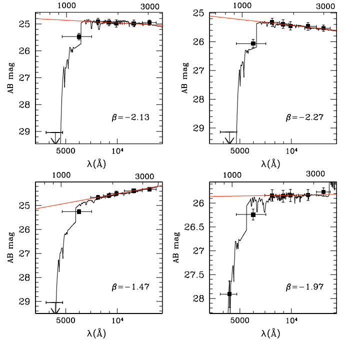
Fig. 3. A comparison of the fitted UV slope (red continuous line) and best-fit SED of four objects in our sample having best-fit photometric redshift in the range z_{phot} = 3.5 - 4.1 . The observed magnitudes (filled squares and errorbars) are, from left to right: B, V, I, Z, Y, J, H. The linear-fit is performed on I, Z, Y, J. The lower and upper horizontal axis show the observer-frame and the rest-frame wavelength, respectively.
