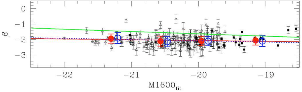
Fig. 9. The \beta - M_{1600} diagram for our B-dropout sample. Open triangles and filled squares represent individual objects in the ERS and HUDF fields, respectively. Errorbars on the observed points are given by the uncertainty on the linear fit on their observed magnitudes. Blue and red circles and lines indicate the result of the statistical analysis described in Sect. 5, which takes into account systematic effects. Blue open circles and errorbars indicate the average \langle\beta\rangle and intrinsic r.m.s of the best-fit Gaussian distributions in each of the four bins: uncertainties on \langle\beta\rangle are much lower and they are not visible in this scale. Red filled circles for the best-fit log-normal distributions. The Gaussians best-fit values are plotted at the average magnitude of the observed points in the relevant bins, log-normal ones with a small magnitude offset for clarity. The green continuous line is the \beta - UV relation by Bouwens et al. (2009). We show for comparison a linear fit on the Gaussian and log-normal best-fit points (blue dashed and red continuous lines): we underline however that our analysis indicates a significant difference only between the first and second magnitude bins.
