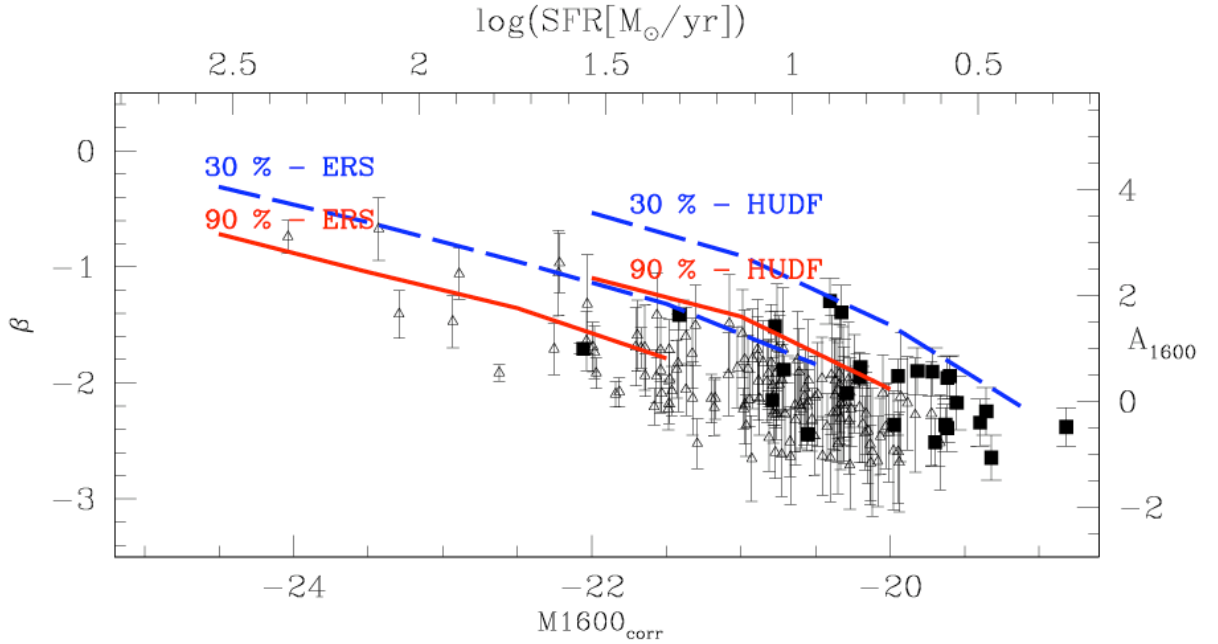
Fig. 10. The relation between \beta and the dust-corrected UV magnitude for ERS (open triangles) and HUDF objects (filled squares) in our sample. The upper and the right axes show the conversion of unextinguished magnitude and UV slope in SFR (Madau et al. 1998) and A_{1600} (Meurer et al. 1999) respectively. The red continuous lines and the blue dashed ones indicate the 90% and 30% selection completeness in the two fields.
