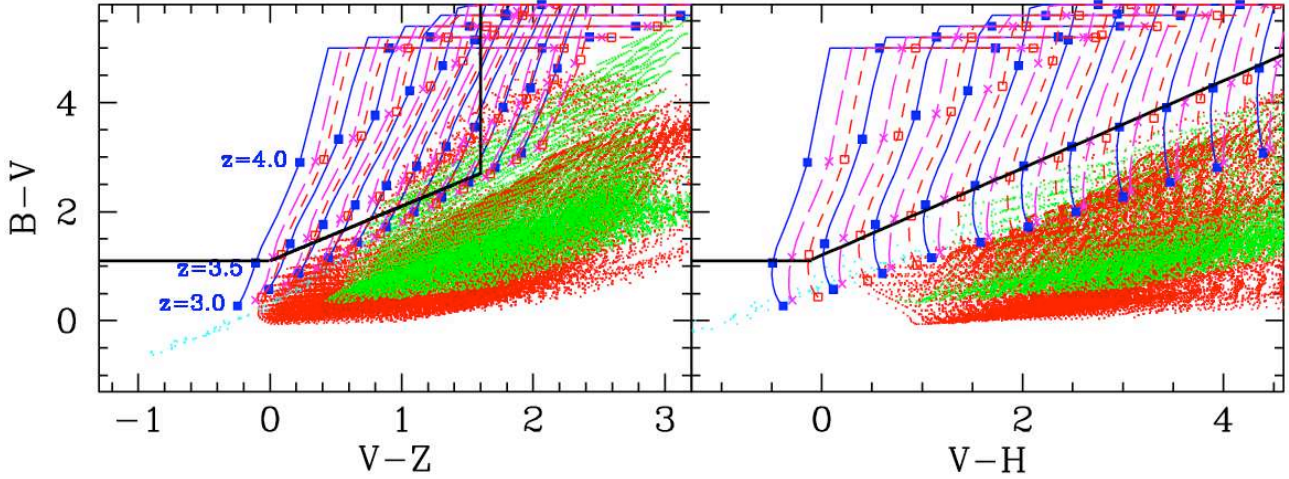
Fig. 1. The (B-V) vs (V-H) colour selection window adopted in the present paper (right) along with the commonly adopted one based on the (V-Z) colour (left). Blue filled squares and lines are for a CB07 LBG model with Z/Z_{\odot} = 0.2 and \text{Age}=100\text{Myr} at increasing redshift and E(B-V) respectively. Models having solar metallicity and \text{Age}=100\text{Myr} and \text{Age}=300\text{Myr} are represented in magenta (crosses and long-dashed lines), and red (empty squares and short-dashed lines), respectively. Red and green points indicate lower redshift passively evolving and dusty star-forming galaxies respectively. See main body for details.
