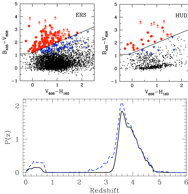
Fig. 2. Upper panels: colour-colour diagrams for B-dropouts in the ERS (left) and HUDF (right) fields. Selected objects are marked in red, the blue points indicate B-dropout candidates in the (B-V) vs (V-Z) selection window excluded by the present analysis. Lower panel: combined photometric redshift probability distribution of our ERS B-dropout candidates (black line) and of galaxies selected from the (B-V) vs (V-Z) diagram (blue dashed line): the (V-H) selected objects have a lower probability of having z_{\text{phot}} \lesssim 3.5 solutions.
