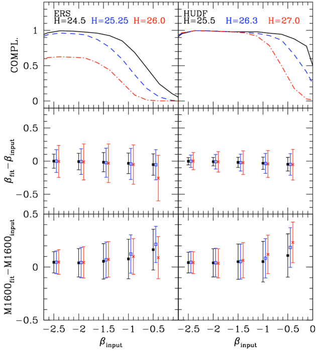
Fig. 7. From top to bottom: detection completeness and difference between output and input \beta and M_{1600} from our ERS (left) and HUDF (right) mock catalogues. All quantities are computed for objects in three observed magnitude bins centred at: H=24.5 (ERS) and H=25.5 (HUDF) (black continuous lines and filled squares); H=25.25 (ERS) and H=26.3 (HUDF) (dashed blue lines and open squares); H=26.0 (ERS) and H=27.0 (HUDF) (red dot-dashed lines and crosses).
