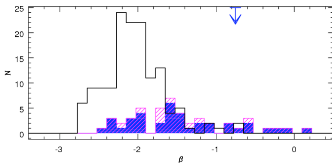
Fig. 6. Distribution of the UV slope values from the ERS sample (black hollow histogram). The magenta dashed histogram represent the objects that are not included in our sample but are selected through a standard (V-Z) colour-cut: most of them have z_{phot} < 3.5 (blue filled histogram). The blue arrow marks the position of a z_{spec} = 3.11 object included in this last sample.
