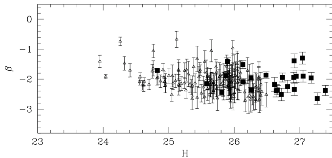
Fig. 5. The UV slope \beta of the ERS (open triangles) and HUDF (filled squares) B-dropout objects as a function of their observed H band magnitude. Errorbars are given by the uncertainty on the linear fit to their observed I, Z, Y, J AB magnitudes.
