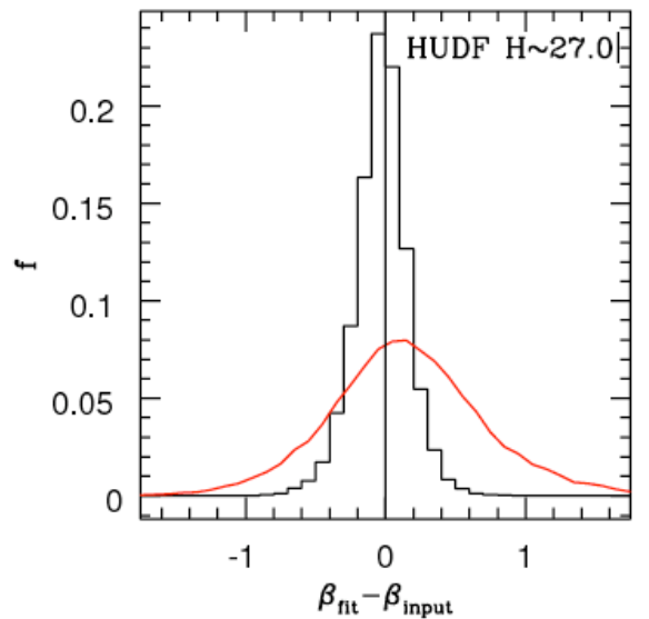
Fig. 4. Comparison of uncertainties on \beta derived from a linear fit to the observed I, Z, Y, J magnitudes (histogram) and from the (I-Z) colour only (red curve) for simulated objects with observed UV slope \beta_{fit} . The real UV slope \beta_{input} of each model is measured on its unperturbed magnitudes.
