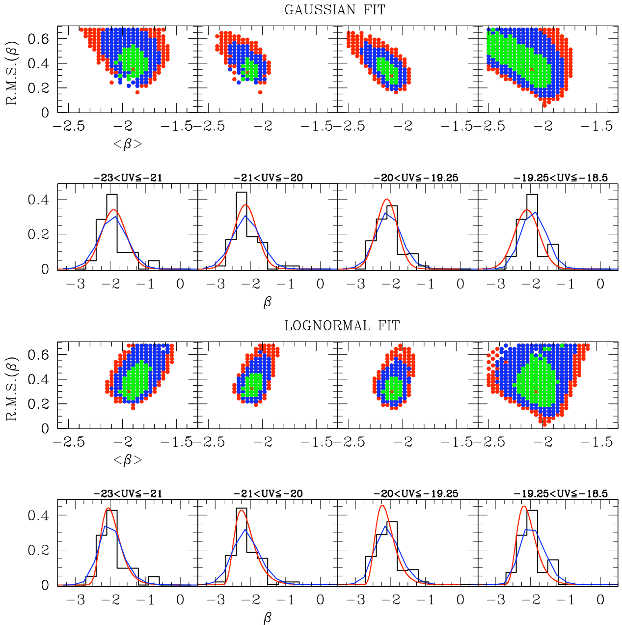
Fig. 8. Maximum likelihood contours (68%, 95% and 99% c.l. in green, blue, and red respectively) for the Gaussian and lognormal fit at different magnitudes. The histograms are the observed data. The red continuous line in each bin is the relevant best-fit distribution. The blue line show how it appears after being “convolved” by observational effects.
