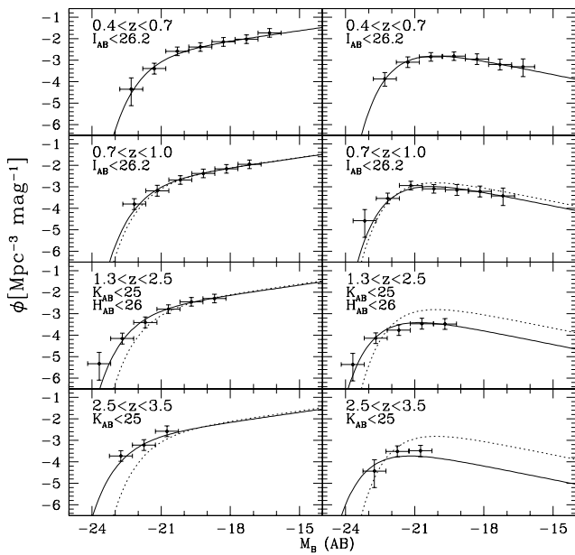
FIG. 8.—LF of blue ( left ) and red ( right ) galaxies separated in the rest-frame U - V color following the S0 evolutionary track (see text for details). Continuous curves come from the maximum likelihood analysis. The LF in the lowest redshift bin 0.4 < z < 0.7 is also shown for comparison in all panels ( dotted curve ).
