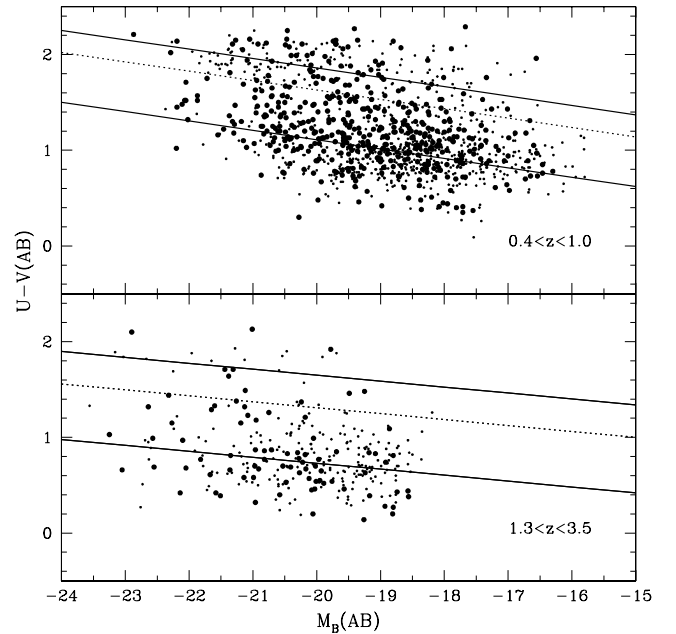
FIG. 3.—Color-magnitude relation in two redshift intervals. Black filled circles represent galaxies with E(B - V) \geq 0.2 . Small dots represent galaxies with E(B - V) < 0.2 . Thick lines represent the best-fit relations for the red and blue populations. Dotted lines represent the locus of the minimum between the two distributions used for the class separation.
