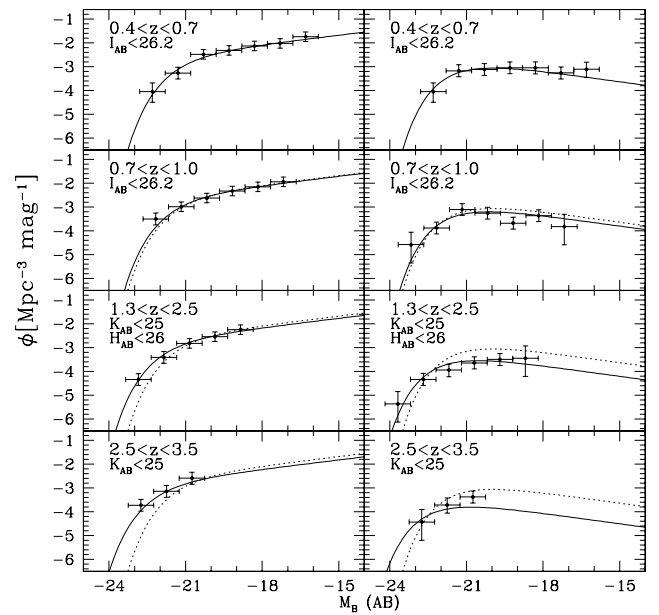
FIG. 9.—LF of late ( left ) and early ( right ) galaxies separated on the basis of their SSFR \dot{m}_*/m_* following the S0 evolutionary track. The LF in the lowest redshift bin 0.4 < z < 0.7 is also shown for comparison in all panels ( dotted curve ).
