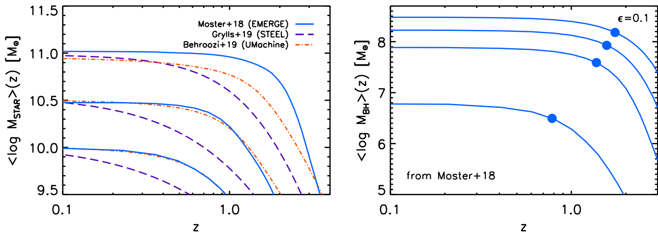
Figure 3. Left: Examples of average stellar mass growth histories M_{\text{star}}[z] from Moster et al. (2018), Grylls et al. (2019b), and Behroozi et al. (2018), as labelled. Right: Examples of average black hole mass accretion histories M_{\text{bh}}[z] as expected from the mean X-ray luminosities of Figure 1, assuming a radiative efficiency of \epsilon = 0.1 and the Moster et al. (2018) stellar mass growth histories. The filled circle on each black hole mass track marks the redshift at which the black hole reaches 50% of its final mass. Lower mass black holes gain more of their mass at late times, the behaviour often referred to as “downsizing”.
