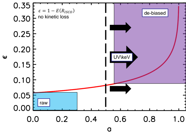
Figure 7. Radiative efficiency as a function of black hole spin (solid, red line) for direct accretion assuming no kinetic losses and \varepsilon = 1 - E with E the energy at the innermost stable circular orbit (Bardeen et al. 1972). The constraints on the mean radiative efficiency arising from the fit to the intrinsic/unbiased M_{\text{bh}}-M_{\text{star}} relation, \varepsilon \gtrsim 0.1 (with dimensionless spin parameter a \gtrsim 0.5 ), are shown with a purple rectangle, while those from the observed M_{\text{bh}}-M_{\text{star}} relation, \varepsilon \lesssim 0.05 , are shown with a cyan rectangle. The independent estimates of the spin parameter from UV/X-ray spectral modelling (black arrows) are broadly consistent with the former estimates with a \gtrsim 0.5 .
