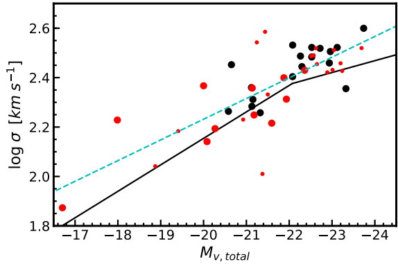
Figure A1. Same layout as Figure 2 in Kormendy (2019). Comparison between the double power-law local \sigma-M_V relation (solid black line) by Lauer et al. (2007) and Kormendy & Bender (2013), with the Kormendy (2019) data set of galaxies with dynamical measurements of their central supermassive black hole mass subdivided into core (black circles) and coreless (red circles) galaxies. The long-dashed, cyan line is a linear fit to the Kormendy (2019) black hole data, proving that at fixed (total) galaxy magnitude M_V , local black holes’ hosts tend to have larger mean velocity dispersions than the underlying population of local galaxies.
