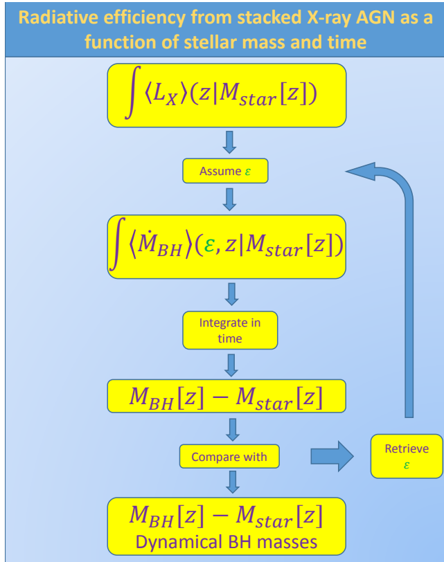
Figure 2. Cartoon visualizing the strategy of this work. After assuming a constant radiative efficiency \epsilon , average black hole accretion histories are extracted from the X-ray luminosities as a function of host galaxy stellar mass and redshift averaged over the entire active and non active populations. We then follow input stellar mass growth histories M_{star}[z] , which are converted to black hole mass accretion histories via L_x(z, M_{star}) and \epsilon . The comparison with the local dynamically-based M_{bh} - M_{star} relations (or at any redshift z < 2 in which they are measured) can effectively constrain the input radiative efficiency, in ways largely independent of the obscured fraction of AGN (see text for details).
