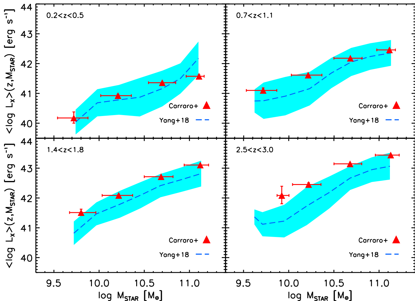
Figure 1. X-ray luminosities, averaged over active and inactive galaxies, as a function of stellar mass and redshift. Data are from Yang et al. (2018) and Carraro et al. (2019, submitted), as labelled. The cyan region brackets the 1\sigma scatter around the mean.
