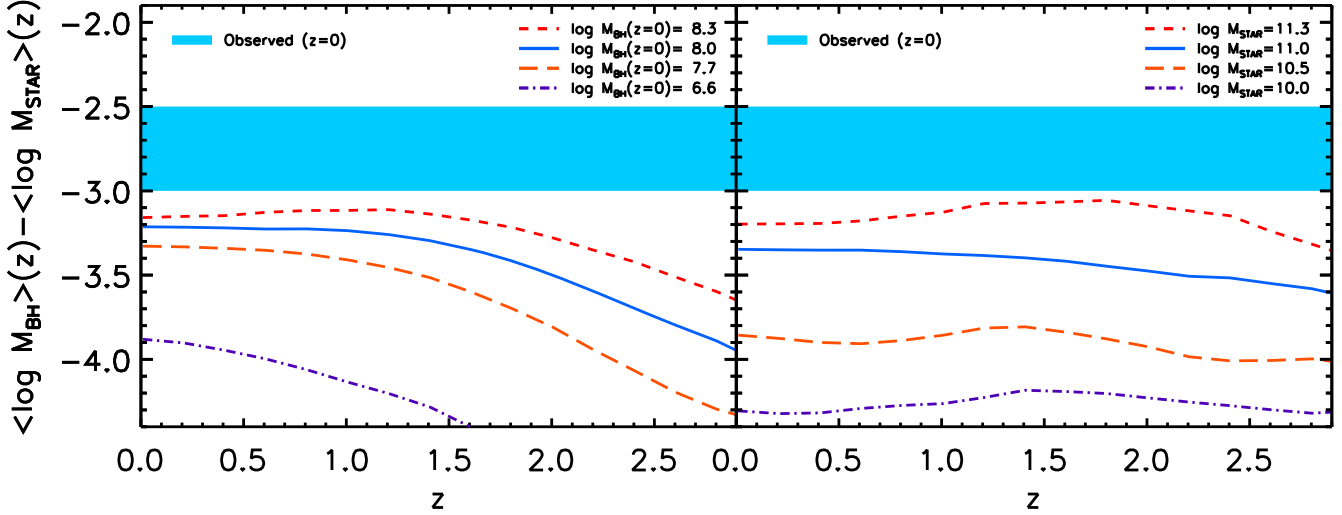
Figure 4. Examples of average black hole-to-stellar mass ratios as a function of redshift along the progenitors (left panel) and at fixed stellar mass (right panel), compared to the average ratio inferred by Kormendy & Ho (2013) in the local Universe (cyan region). At each M_{\text{star}} in the right panel, the ratio \langle M_{\text{bh}} \rangle / \langle M_{\text{star}} \rangle is roughly constant, at least for z < 2 .
