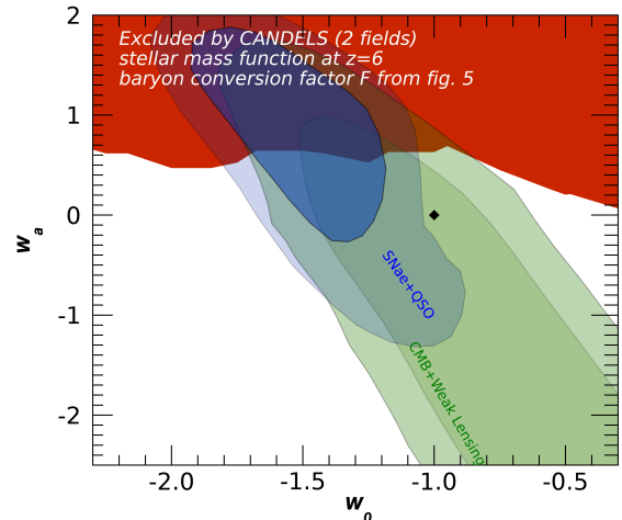
Fig. 6. As in fig. 2, but assuming the baryon efficiency F from fig. 5.
