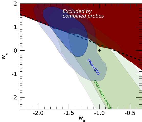
Fig. 10. Exclusion regions ( 2\text{-}\sigma confidence level) in the w_0 - w_a plane derived from combining the different probes. For each observable, the most conservative case has been considered: for the CANDELS field we have assumed F = 0.5 , for SPT031158 we have taken a DM mass M = 2 \cdot 10^{12} M_\odot , and for submm galaxies we have converted stellar masses to DM mass assuming M = M_*/f_b . The dashed line shows the analytical approximation for the boundary of the excluded region w_a = -3/4 - (w_0 + 3/2) .
