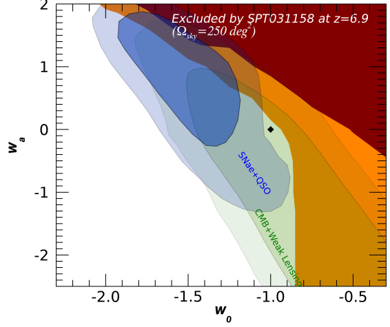
Fig. 9. Same as fig. 8, but assuming an effective SPT area \Omega_{\text{sky}} = 250 \text{ deg}^2 .
