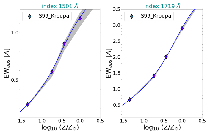
Fig. 2. Diagrams showing the dependence between equivalent width (EW) and metallicity for the 1501 and 1719 Å absorption line indexes that we adopt in this paper according to Starburst99 models. All the data points are derived assuming a constant SFH for 100 Myr and Kroupa IMF. The gray shaded region around the main relations represents the variation of EW with the IMF (Kroupa-Salpeter) and with the ages of the stellar population chosen (50 Myr - 2 Gyr), as described in the text. The final metallicity calibrations are based on a third order polynomial fit to the data points, and are shown with a blue continuous line in each panel. Their explicit forms are given in the text in Equations 2 and 3.
