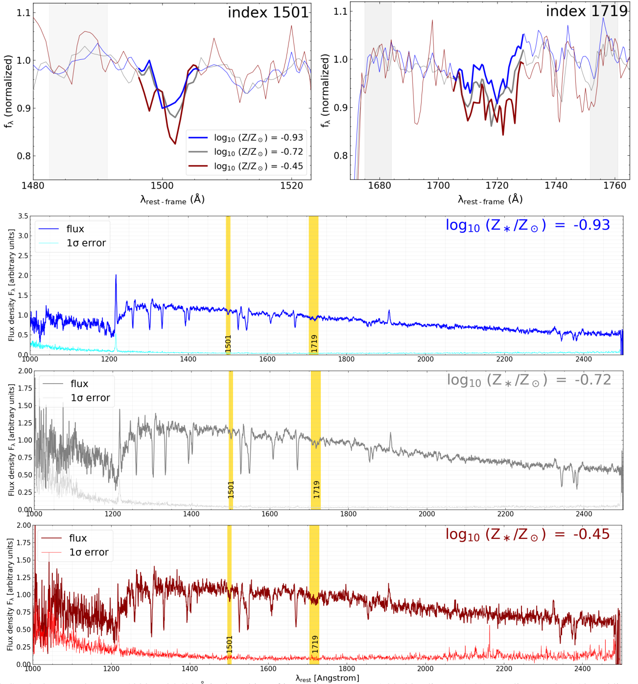
Fig. 9. Stacked spectra between 1000 and 2500 Å in three bins of increasing \beta_{\text{median}} : -1.98 (blue line), -1.51 (gray line), and -1.10 (red line) (see also Table 3). The absorption complexes used in this work to estimate the metallicity, located at 1501 and 1719 Å, are highlighted with yellow vertical bands. In the two top panels, the three stacks are plotted together and zoomed around the two metallicity indexes. A thicker line specifies both the width of each absorption complex, while grey shaded areas indicate the spectral ranges for the estimation of the pseudocontinuum. Spectral stacks of galaxies with redder UV slopes have deeper absorption features, hence higher metallicity.
