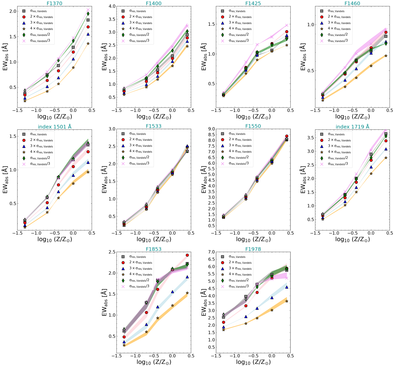
Fig. A.6. Stellar metallicity vs equivalent width predicted by Starbursts99 models for the ten absorption lines studied in this paper and for different spectral resolutions. The resolution elements \sigma_{\text{res}} tested are 1/2, 1/3, 1, 2, 3, and 4 times the VANDELS value. All the symbols are derived with a constant SFH and a stellar age of 100 Myr. The shaded regions allow the stellar age to vary between 50 and 100 Myr.
