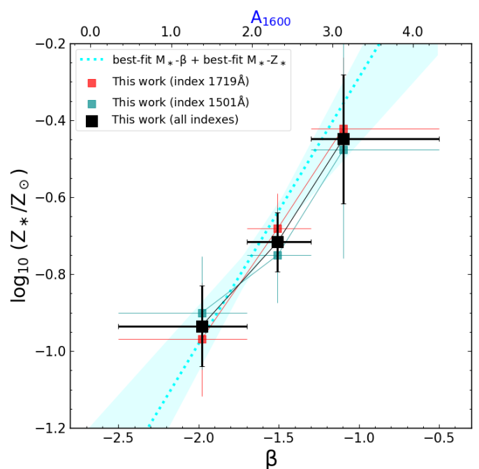
Fig. 8. Relation between the UV slope and the stellar metallicity for VANDELS galaxies. The average relation from the two indexes (1501 and 1719 Å) is drawn with black squares, while the pale colored squares represent the underlying metallicities from single absorption features. Horizontal bars associated to each of the three data points indicate the range of \beta slopes of galaxies in the same bin. The relation obtained from combining the best-fit MZR and the M_* - \beta relation is highlighted with a cyan dashed line and cyan 1\sigma uncertainty area. On the top x-axis, A_{1600} is shown for comparison purposes, as determined from the \beta - A_{1600} conversion of Meurer et al. (1999). We warn that this conversion may also depend at a second order on the metallicity itself.
