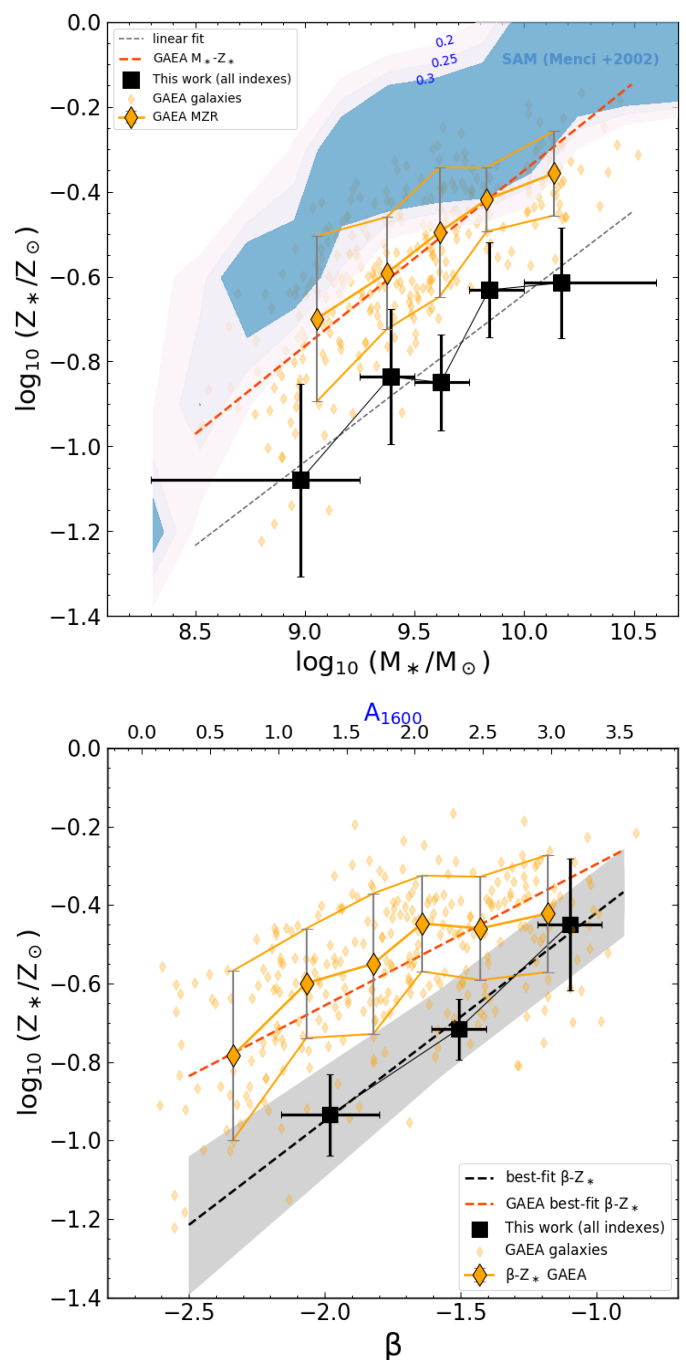
Fig. 10. Top: Comparison between the MZR derived from VANDELS (black squares and error bars) and from predictions of two semi-analytic models: orange diamonds represent the median masses and metallicities of GAEA galaxies in five bins of stellar mass defined as for the observations. Blue contour regions indicate the fraction of galaxies in the SAM of Menci et al. (2014) with different Z_* at a given mass, according to the 2D bins defined in the text. Bottom: Comparison of VANDELS results to the UV slope - metallicity relation predicted by the GAEA models. The orange big diamonds were derived with the same method of the upper panel. We highlight with a black dashed line the best-fit relation for the VANDELS sample, while the gray shaded area encloses its 1\sigma uncertainty region.
