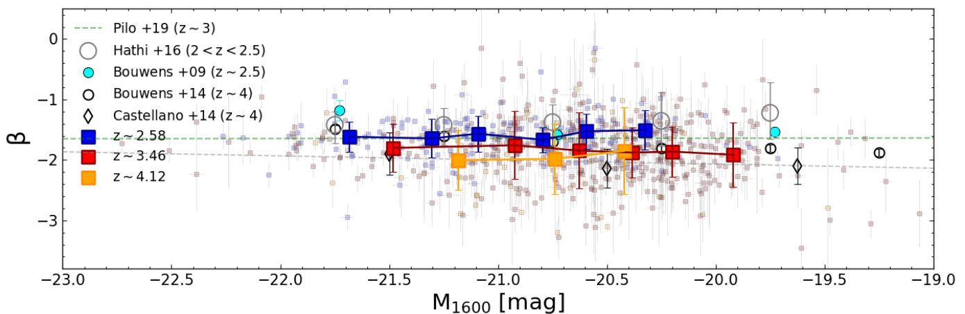
Fig. 1. UV slope vs M_{1600} for VANDELS galaxies selected in this work with \sigma_{\beta} \leq 1 and at least three photometric bands available in the range 1230-2750 Å. Our data are color coded according to three different redshift bins ( 2 < z_{bin1} < 3 < z_{bin2} < 4 < z_{bin3} < 5 in blue, dark-red, and orange, respectively), with z estimated from VANDELS spectra. The median z in each bin is reported in the legend. For comparison are shown the M_{1600} - \beta relations found by Hathi et al. (2016) at 2 < z < 2.5 (gray empty circles), Bouwens et al. (2009) at \sim 2.5 (cyan circles), Bouwens et al. (2014) at \sim 4 (black empty circles), and Castellano et al. (2014) for LBGs at z \sim 4 (black empty diamonds and light-gray dashed best-fit line). The relation found by Pilo et al. (2019) for LBGs at z \sim 3 is displayed as a light-green dashed line.
