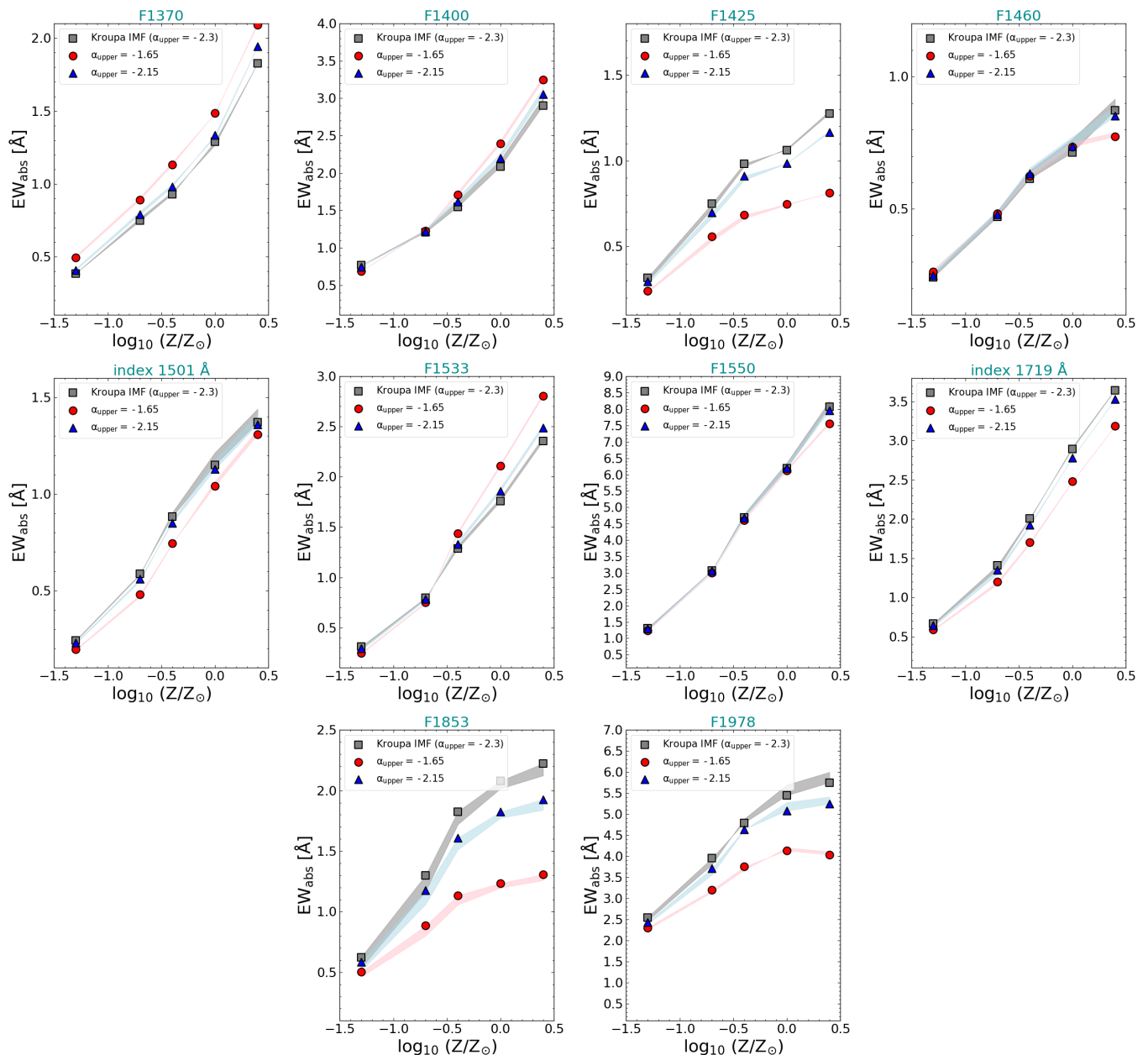
Fig. A.5. Stellar metallicity vs equivalent width predicted by Starbursts99 models for the ten absorption lines studied in this paper. The gray squares are derived assuming a Kroupa IMF ( \alpha_{upper} = -2.3 ), the blue triangles are built by changing the high-mass end slope to \alpha_{upper} = -2.15 (as in Baldry & Glazebrook 2003), while the red circles assume an extremely flat slope \alpha_{upper} = -1.65 . All the symbols are representative of a constant SFH and a stellar age of 100 Myr. The shaded regions allow the stellar age to vary between 50 and 100 Myr. The other details of the models are the same as in Fig. A.2.
