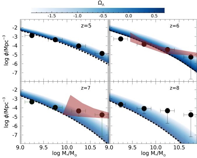
Fig. 6. The stellar mass function of galaxies for the different values of \Omega_\Lambda shown in the color bar for our fiducial combination w_0 = -0.98 , w_a = 0.08 ; the dashed line mark the result for the standard \Lambda CDM cosmology. We compare with the JWST measurements by Weibel et al. (2024) with the estimate by Akens et al. (2024) (shaded area) who considered the additional contribution by LRD under the assumption that their emission is entirely contributed by stars.
